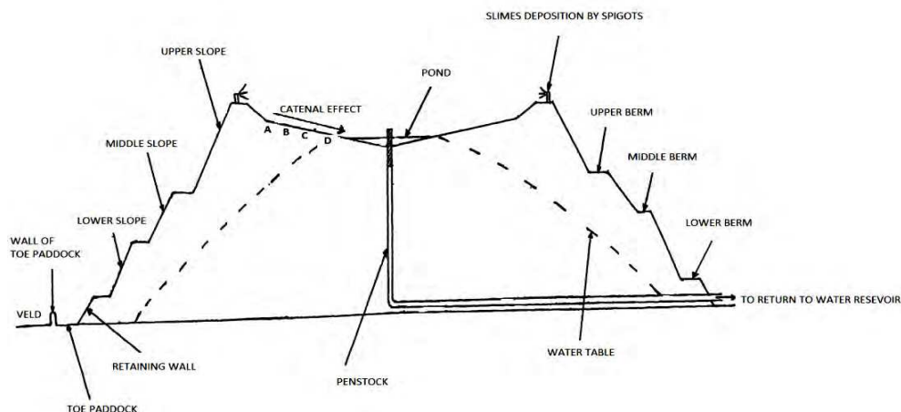
Fig. 7. General section of a TSF.
