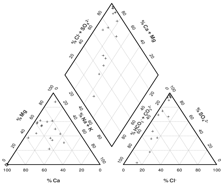
Fig. 15. Distribution of % ( \text{Na}^+ + \text{K}^+ ), % \text{Mg}^{2+} , and % \text{Ca}^{2+} and % \text{Cl}^- , % \text{SO}_4^{2-} , % ( \text{HCO}_3^- + \text{CO}_3^{2-} ) depicting the classification of borehole and surface waters.
